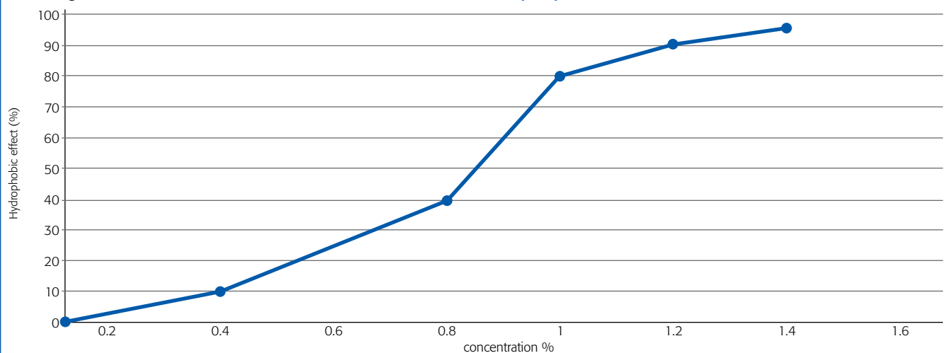
Figure 4: Influence of calcium stearate concentration on the hydrophobic effect of concrete
