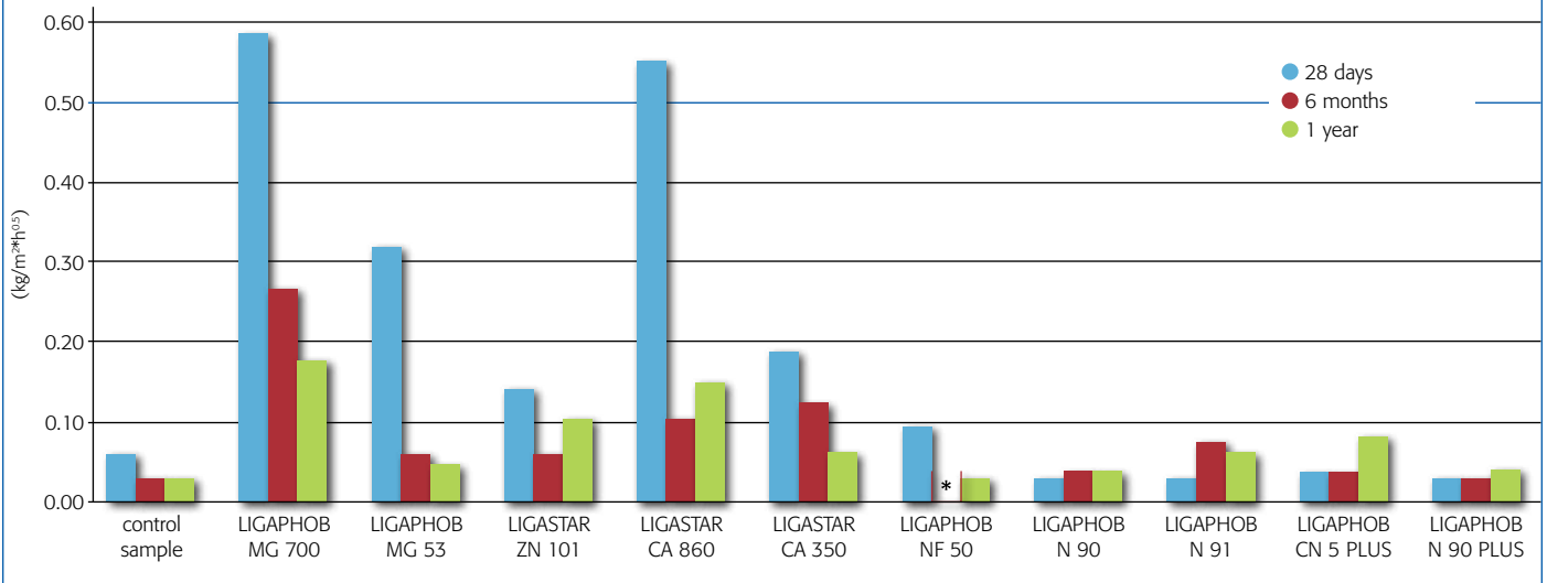
Figure 5: Water absorption/Coefficient
